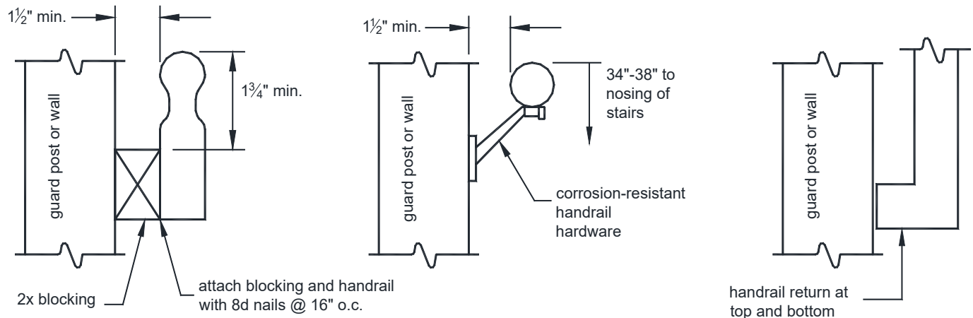
FIGURE 44: HANDRAILS
