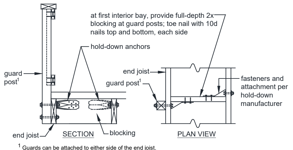
FIGURE 37: GUARD POST-TO-END JOIST
